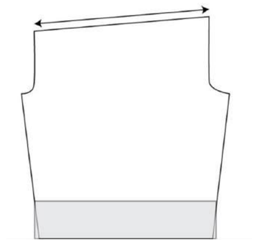
Fig.2.6.11: Pant Drafting
