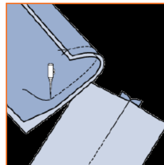
Fig.2.2.6: Superimposed Seams
