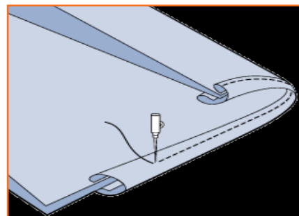
Fig.2.2.8: Bound Seams
