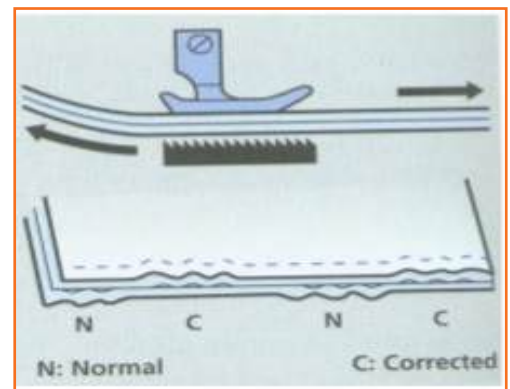
Fig.3.1.8: Feed Pucker
