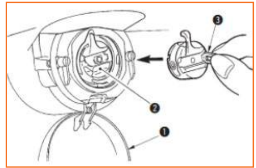
Fig.2.4.18: Installing and removing the bobbin case
