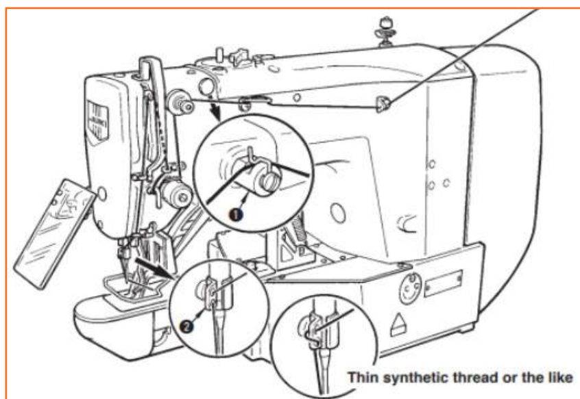
Fig.2.4.17: Threading a bar-tack machine
