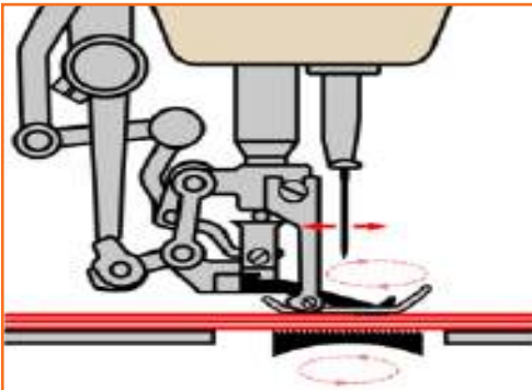
Fig.2.3.44: Unison Feed Mechanism
