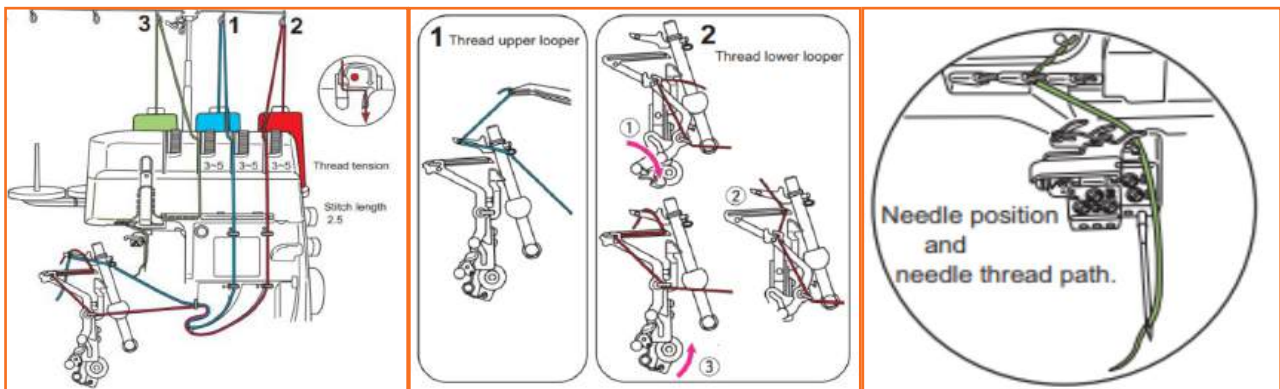
Fig.2.4.1: Threading 3-thread over lock Machine
