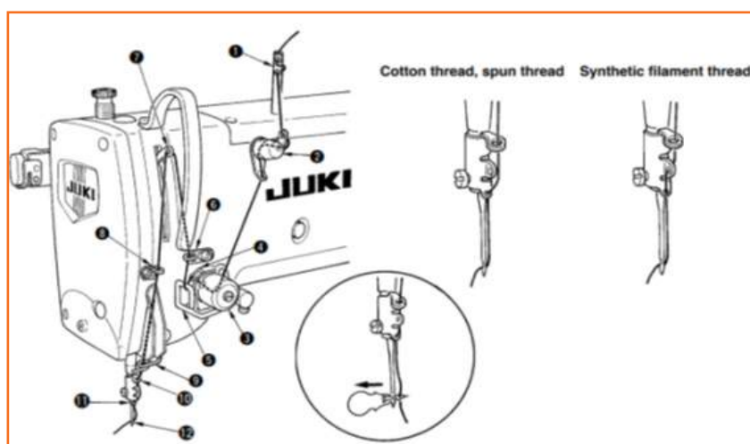
Fig.2.4.34: Threading a button-hole machine
