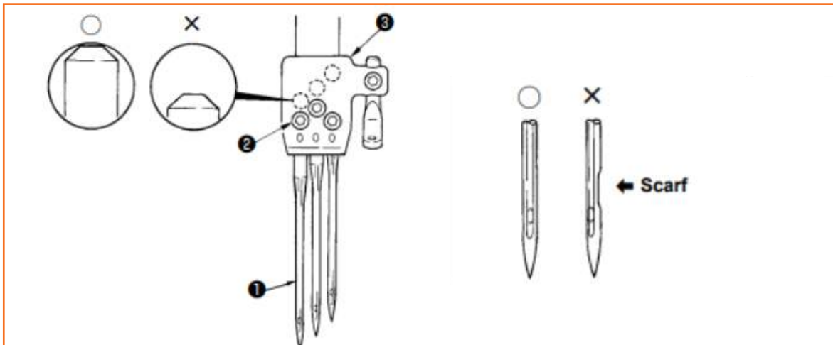
Fig.2.4.7: Changing needle of a flat-lock machine
