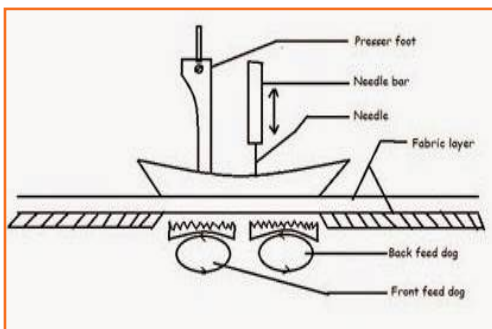
Fig.2.3.40: Differential Bottom Feed Mechanism
