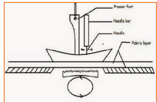
Fig.2.3.43: Needle Feed System Mechanism
