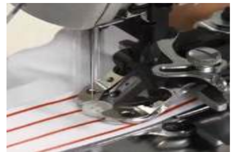
Fig.2.4.31: Operating a Button-attach machine (e)
