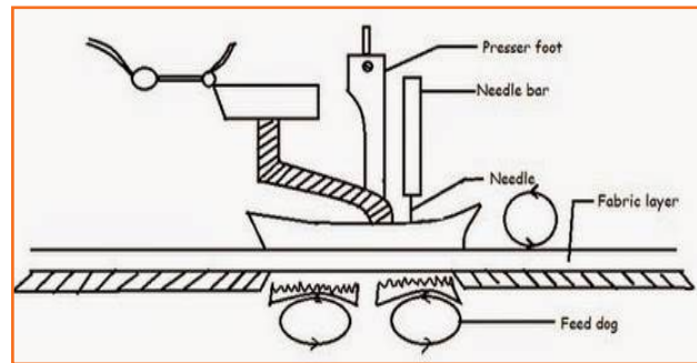
Fig.2.3.42: Differential Bottom Feed Mechanism (b)
