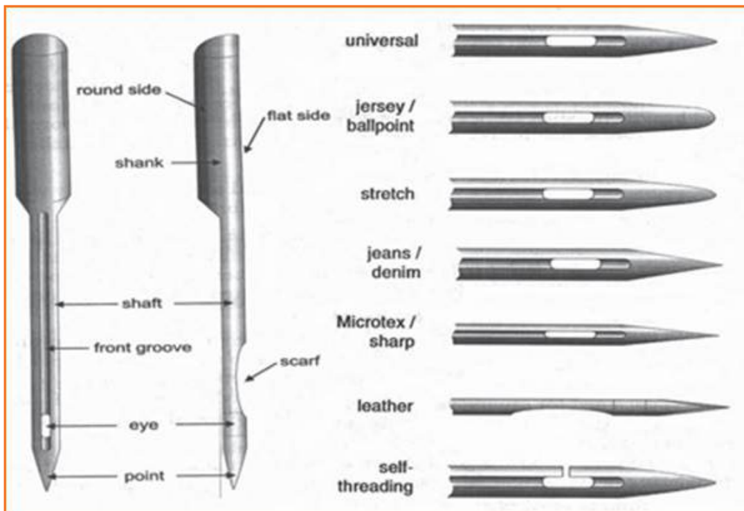
Fig 2.1.42: Parts of a sewing needle
