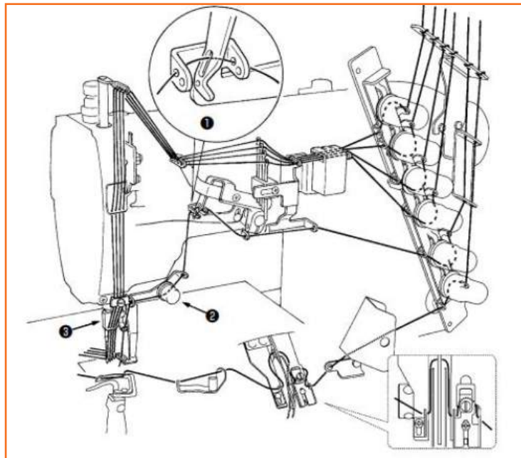
Fig.2.4.8: Threading a Flat Lock Machine
