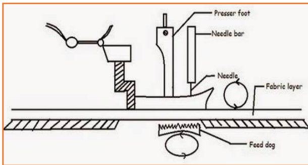
Fig.2.3.41: Differential Bottom Feed Mechanism (a)
