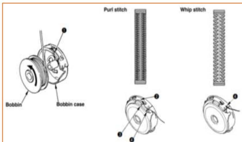
Fig.2.4.35: Threading the bobbin case of a button-hole machine
