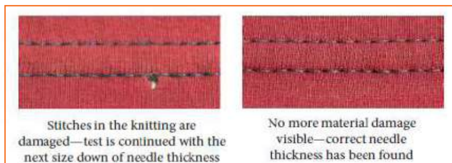
Fig.2.1.44: Choosing Needle Thickness
