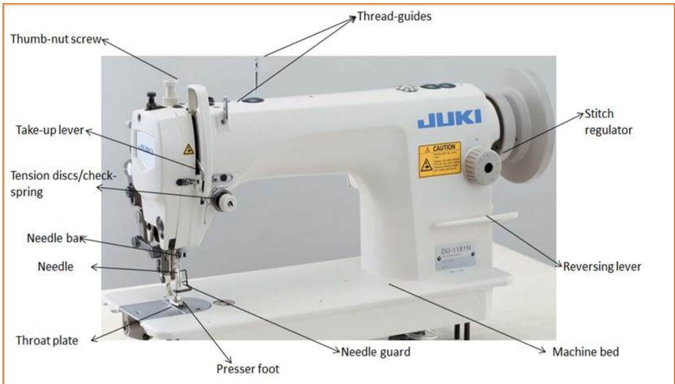
Fig.2.3.2: Parts of a Sewing Machine
