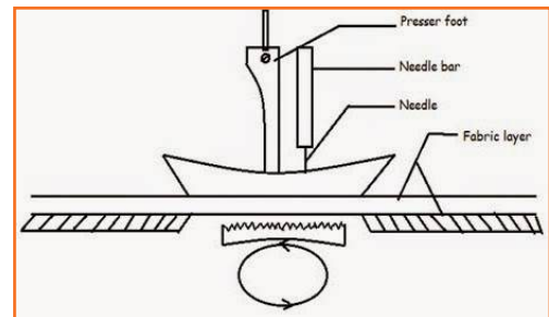
Fig.2.3.39: Drop Feed Mechanism
