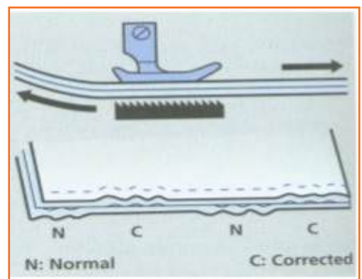
Fig.3.1.8: Feed Pucker
