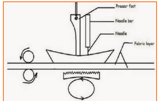
Fig.2.3.45: Puller Feed Mechanism
