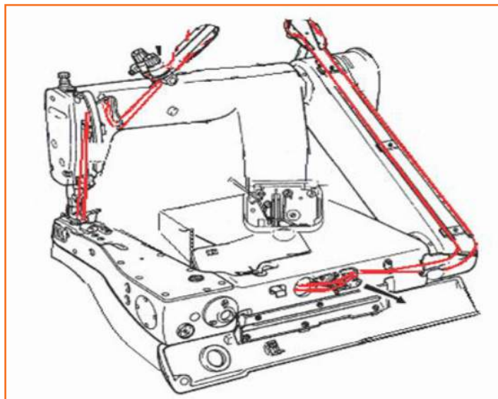
Fig.2.4.39: Changing needle of a button-hole machine
