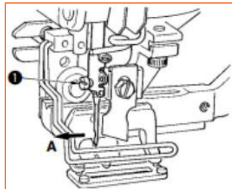
Fig.2.4.33: Changing needle of a button-hole machine
