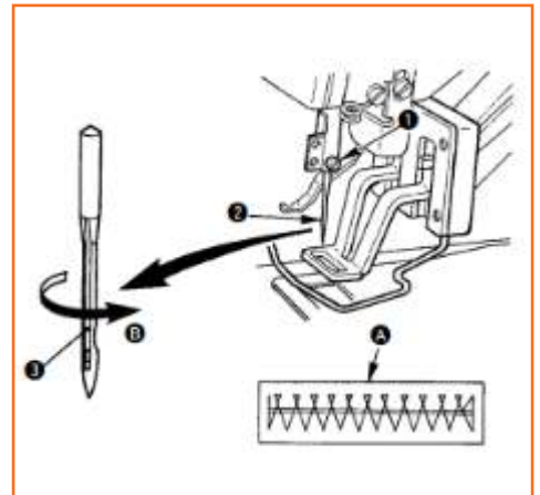
Fig.2.4.16: Changing needle of a bar-tack machine
