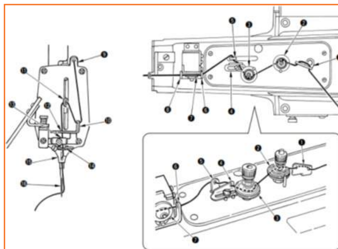
Fig.2.4.26: Threading of Button attach machine
