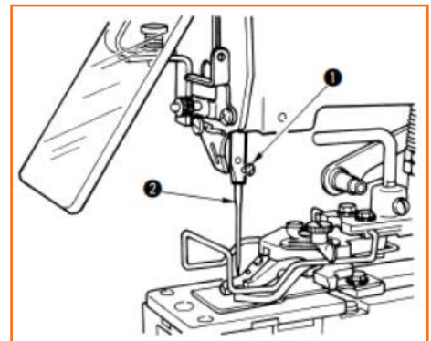
Fig.2.4.25: Changing needle of a button-attach machine
